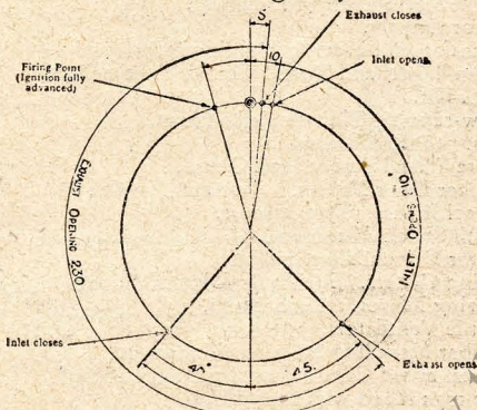
Timing Diagram.
